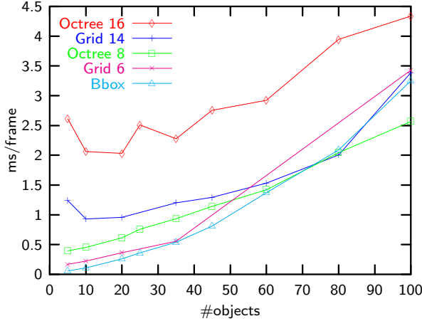
Figure 4: Comparison of grid, octree, and n^2 bounding box tests. The graph labeled “grid 14” corresponds to a grid with 14^3 cells; similarly for the other graphs.
